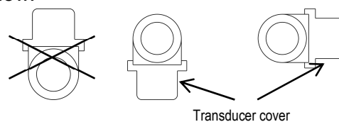
Fig. 9: Recommended installation orientation for cooling metering
